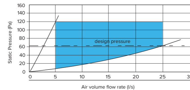
Performance envelope for CVD100
