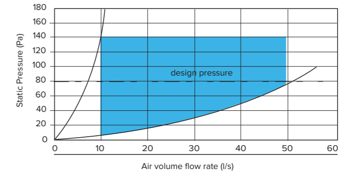
Performance envelope for CVD125
